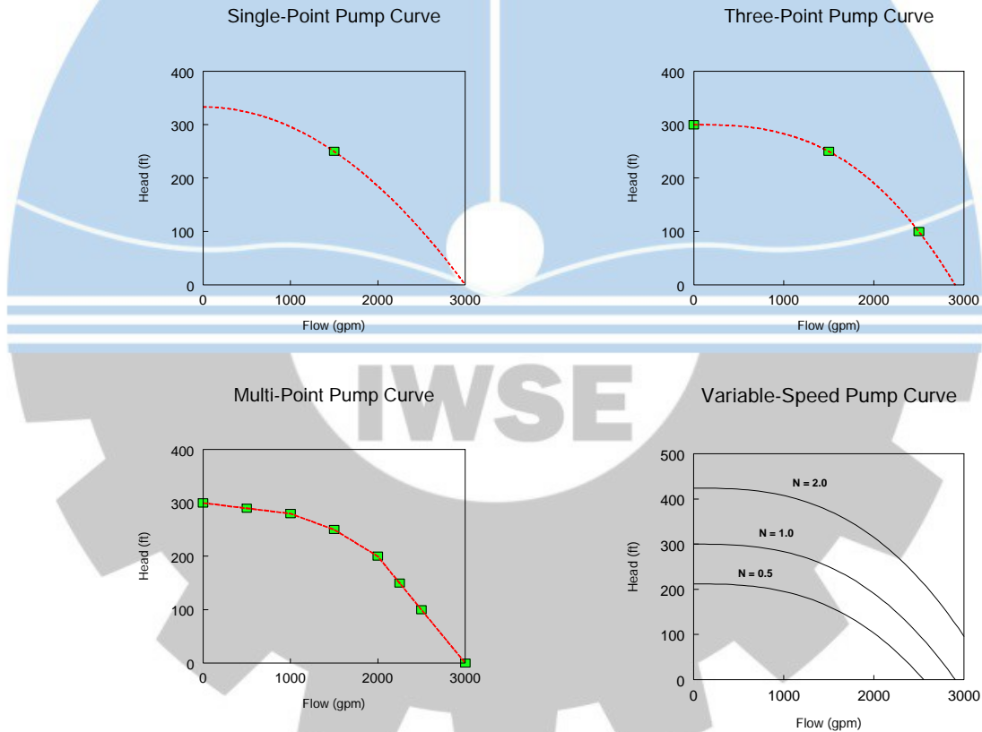
Figure 3.2 Example Pump Curves
