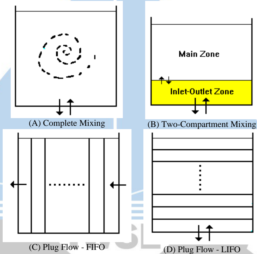
Figure 3.5 Tank Mixing Models
