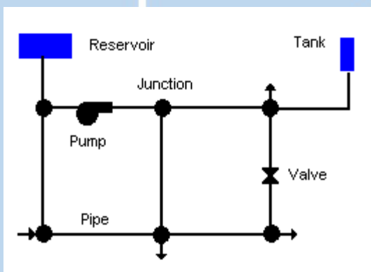
Figure 3.1 Physical Components in a Water Distribution System
