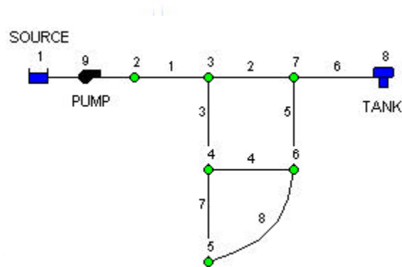
Figure 2.1 Example Pipe Network
