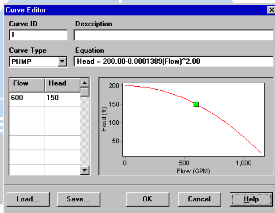
Figure 6.1 Curve Editor
