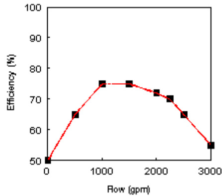
Figure 3.3 Pump Efficiency Curve
